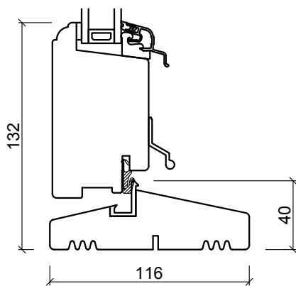
Bottenkarm
