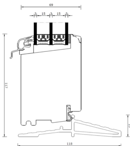
Glasfiber bottenkarm
