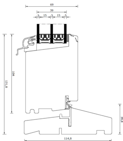
Glasfiber bottenkarm
