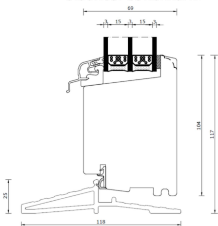
Glasfiber bottenkarm
