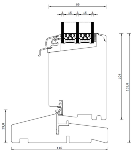
Glasfiber bottenkarm
