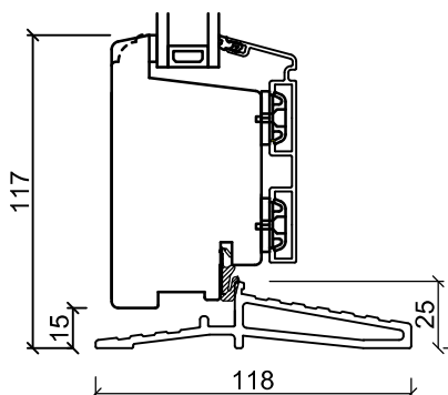
Glasfiber Bottenkarm
