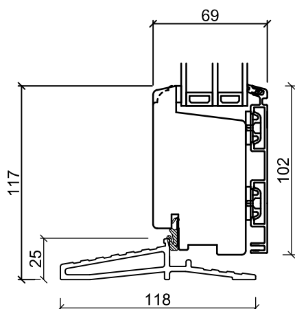
Glasfiber Bottenkarm
