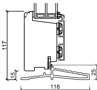
Glasfiber Bottenkarm
