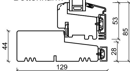
Bottenkarm
