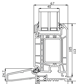
Alu Bottenkarm
