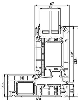
PVC Bottenkarm
