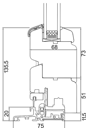
Alu bottenkarm
