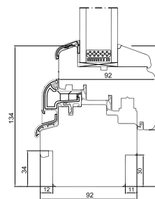
Bottenkarm
