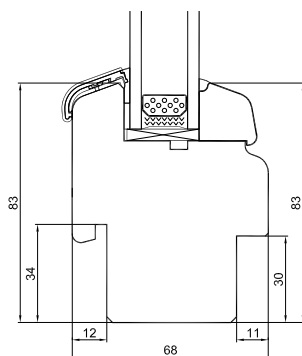
Bottenkarm
