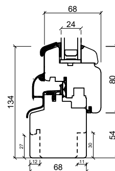
Bottenkarm
