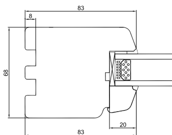
Bottenkarm
