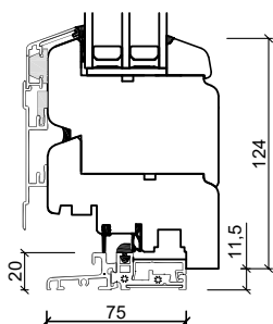
Alu bottenkarm
