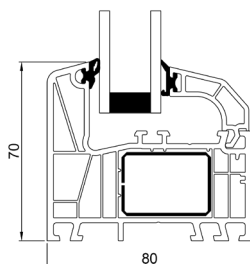
Bottenkarm
