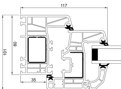
Bottenkarm
