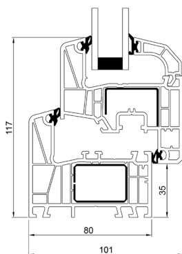
PVC Bottenkarm
