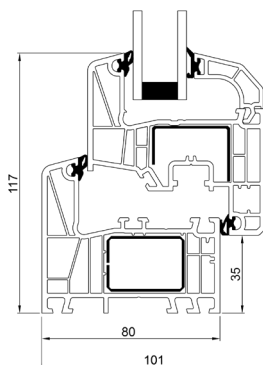
Bottenkarm
