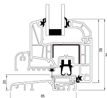
Alu Bottenkarm
