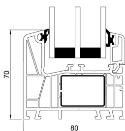
Bottenkarm
