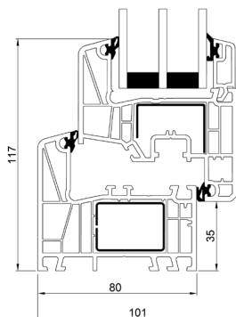
PVC Bottenkarm
