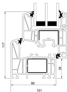
Bottenkarm
