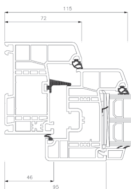
Bottenkarm
