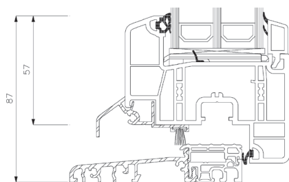
Alu Bottenkarm
