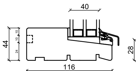
Bottenkarm
