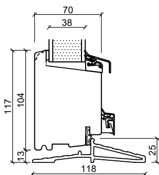
Fiber bottenkarm
