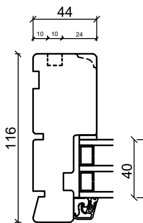
Bottenkarm
