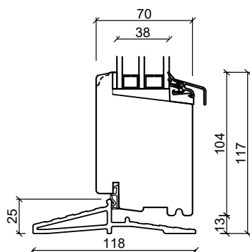
Fiber bottenkarm
