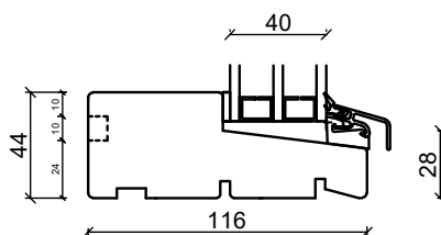
Bottenkarm
