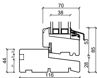
Bottenkarm
