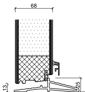
Fiber bottenkarm
