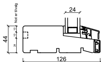
Bottenkarm
