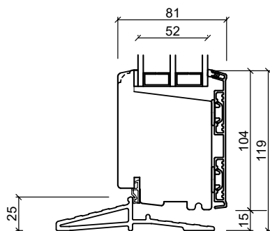
Fiber bottenkarm
