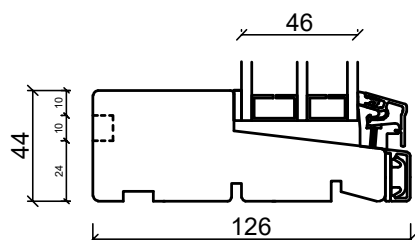
Bottenkarm
