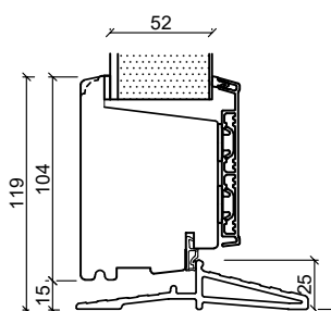
Fiber bottenkarm
