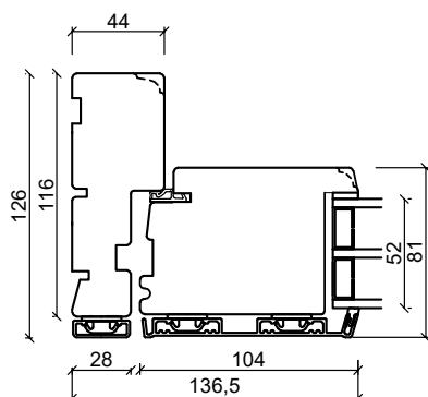
Fiber bottenkarm
