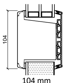
Fiber bottenkarm
