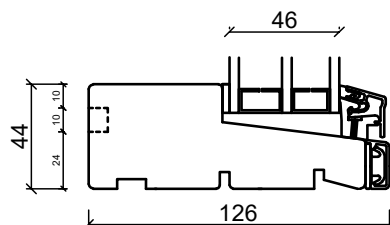
Bottenkarm
